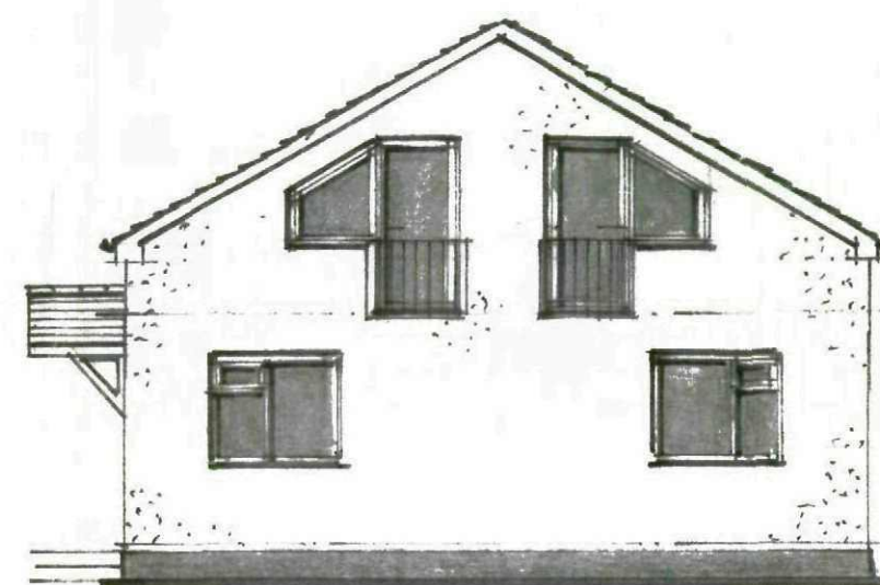
Proposed Front Elevation On 2
