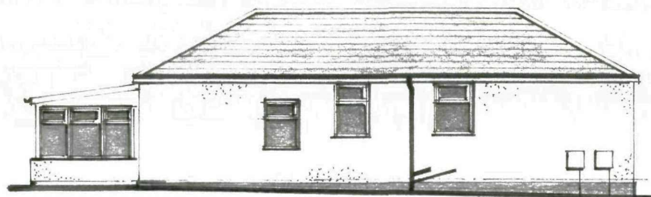
Existing Side Elevation On 1
