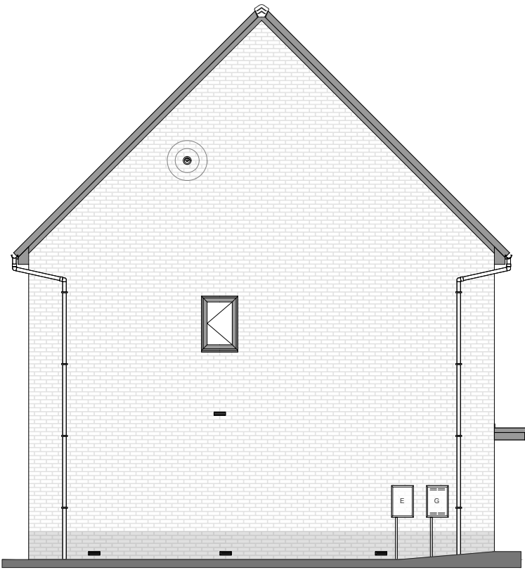
LEFT ELEVATION
