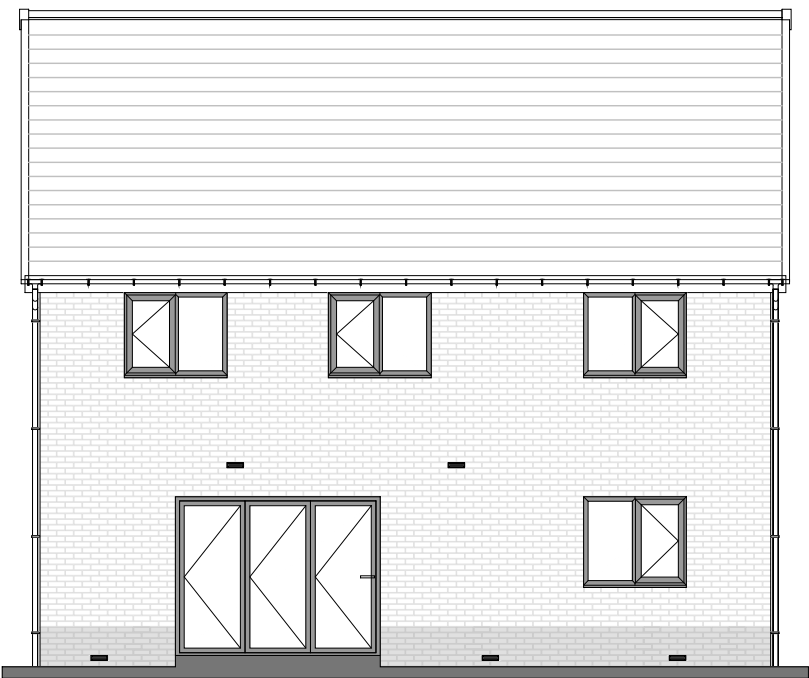
REAR ELEVATION
