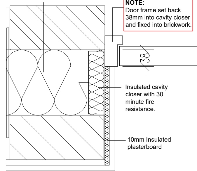
External Door Jamb Detail Scale @ 1:5
