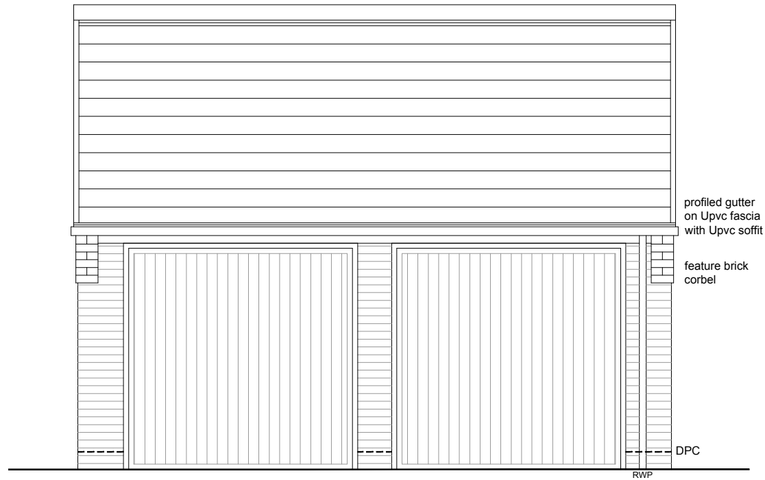
FRONT ELEVATION
