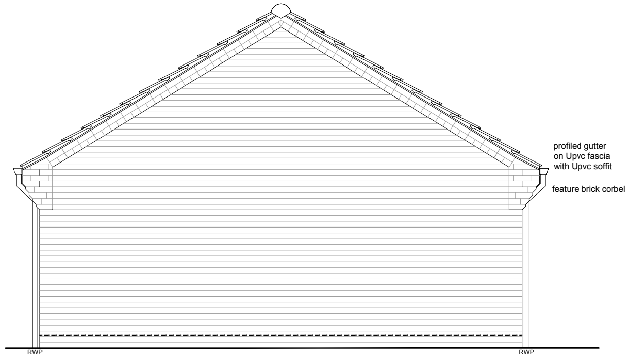
SIDE ELEVATION (SAME BOTH SIDES)
