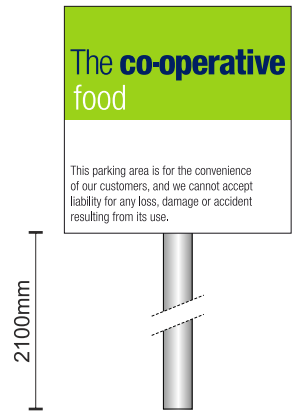
Sign G - Scale 1:20
