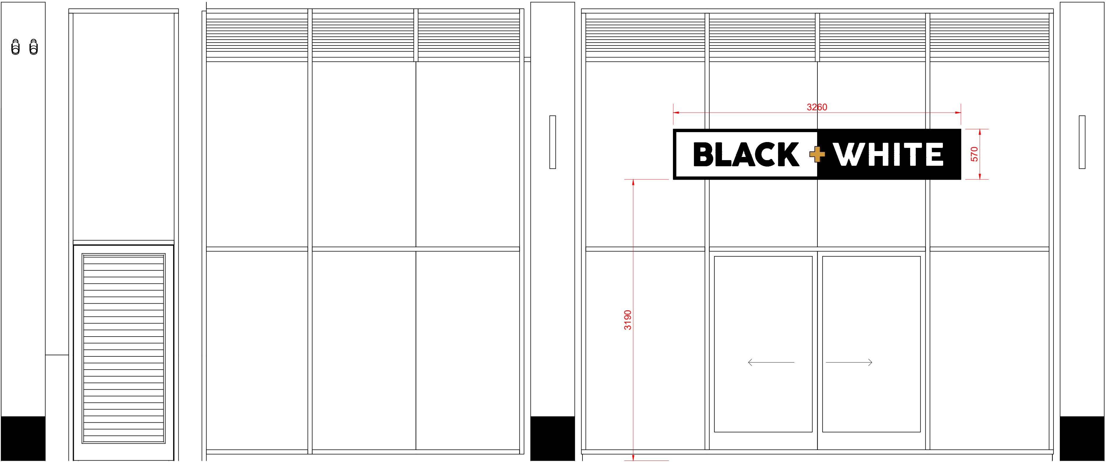
PROPOSED EXTERNAL ELEVATION SCALE 1:25
