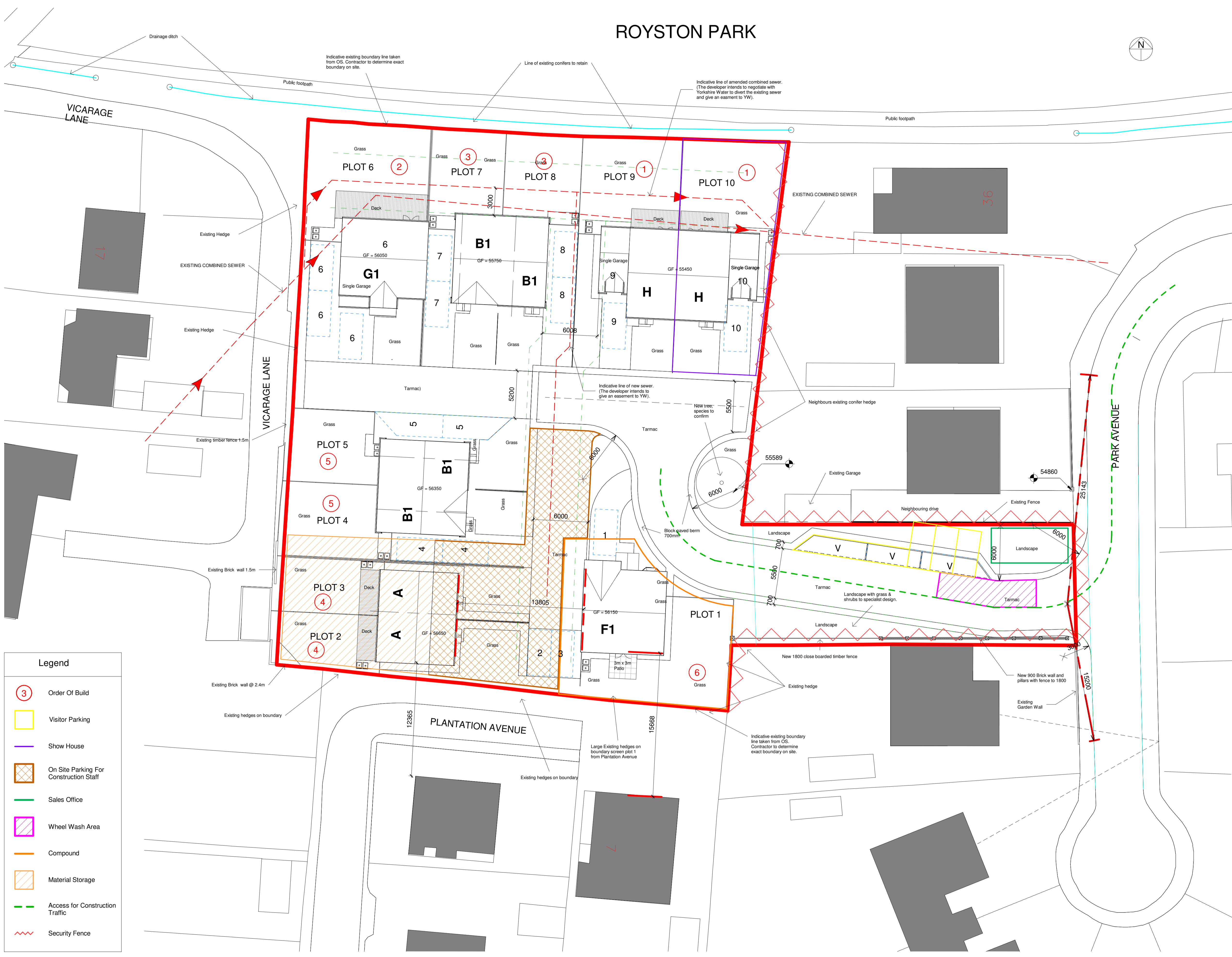
Site Compound Layout 1 : 200
