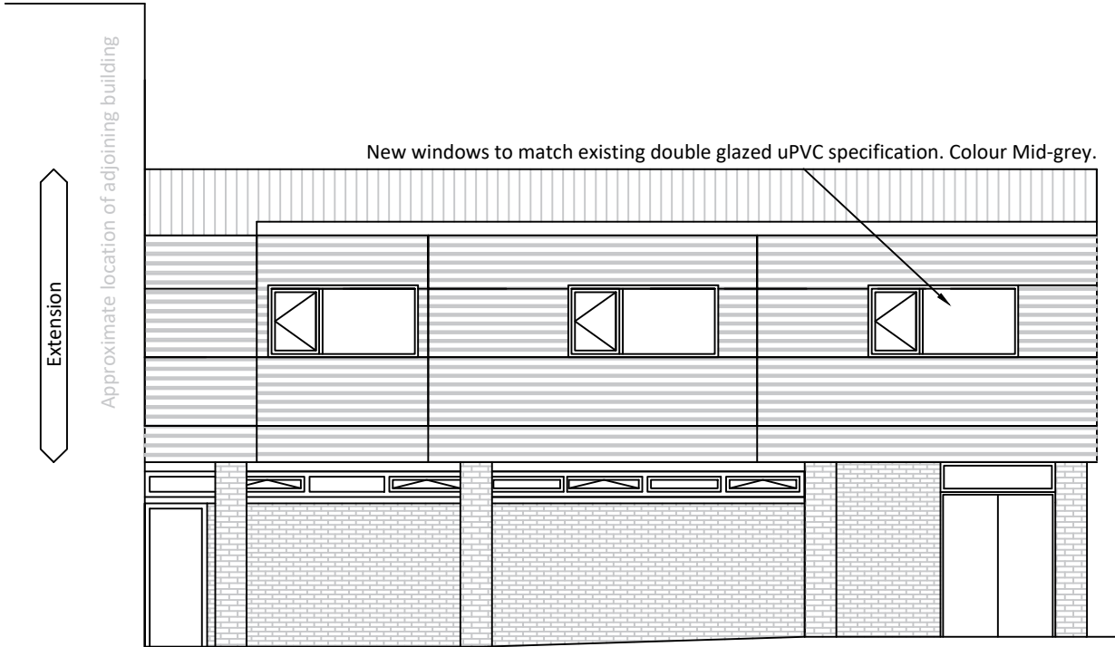
North Elevation
