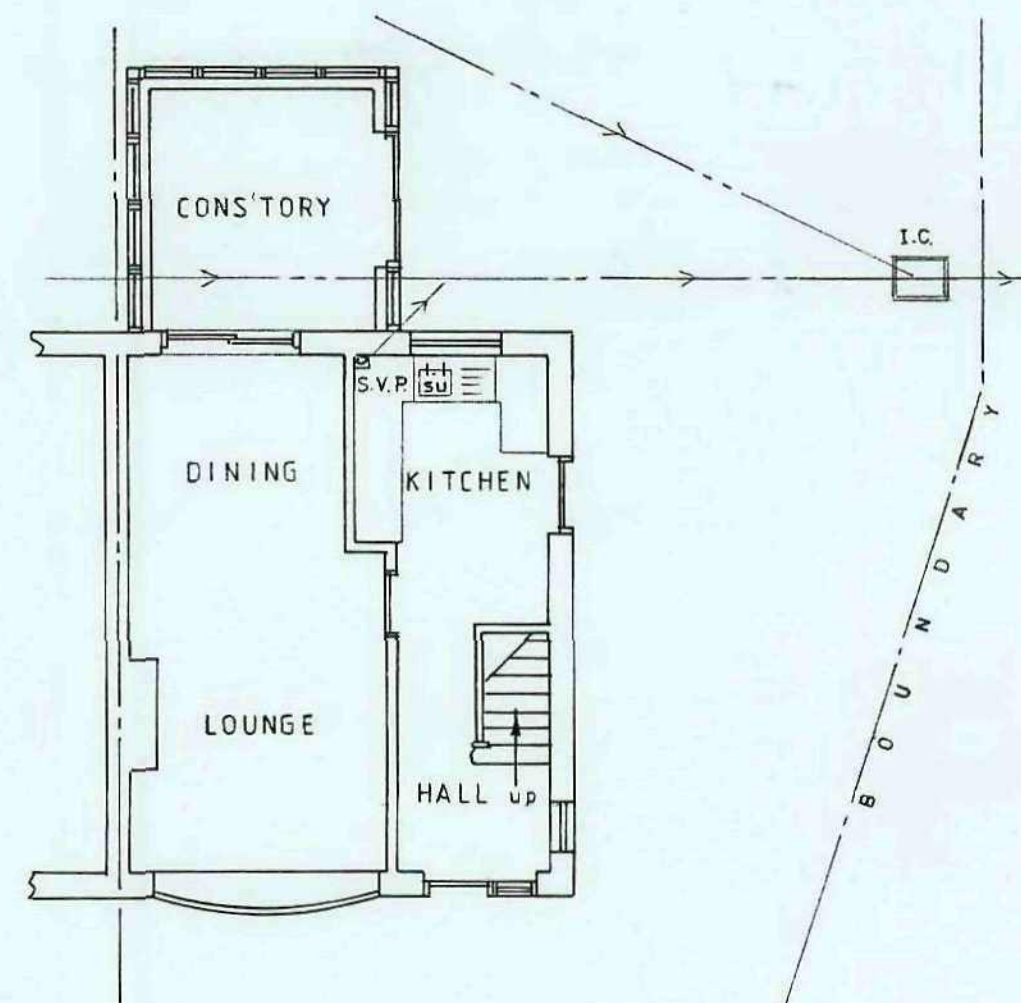
EXISTING G.F. PLAN
