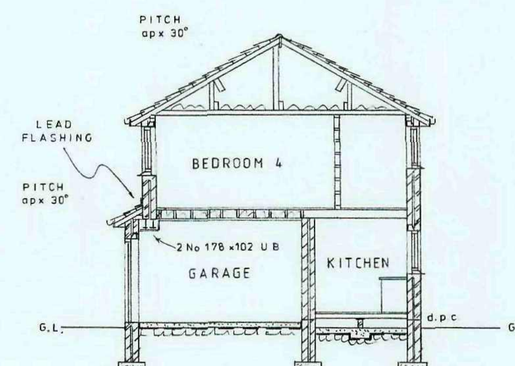
SECTION
