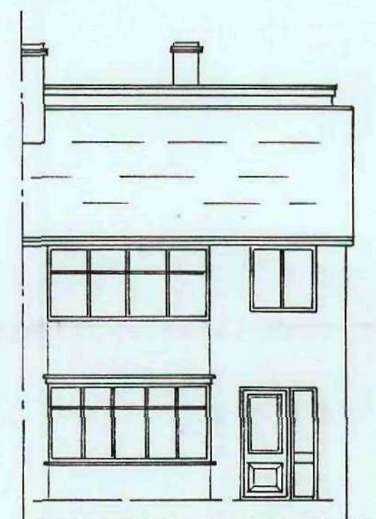
EXISTING FRONT
