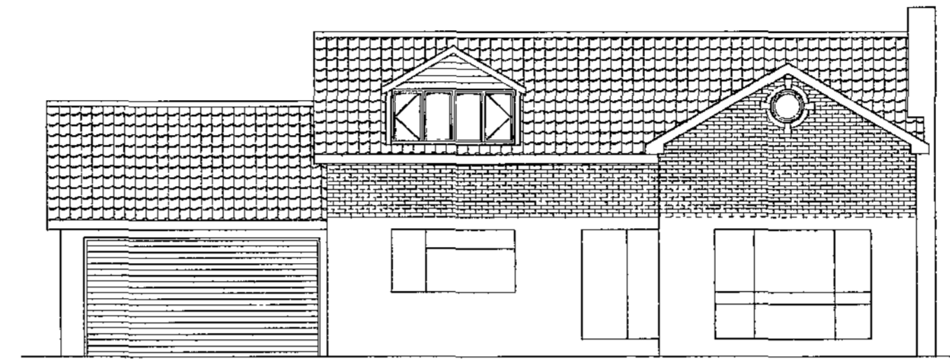
FRONT ELEVATION
