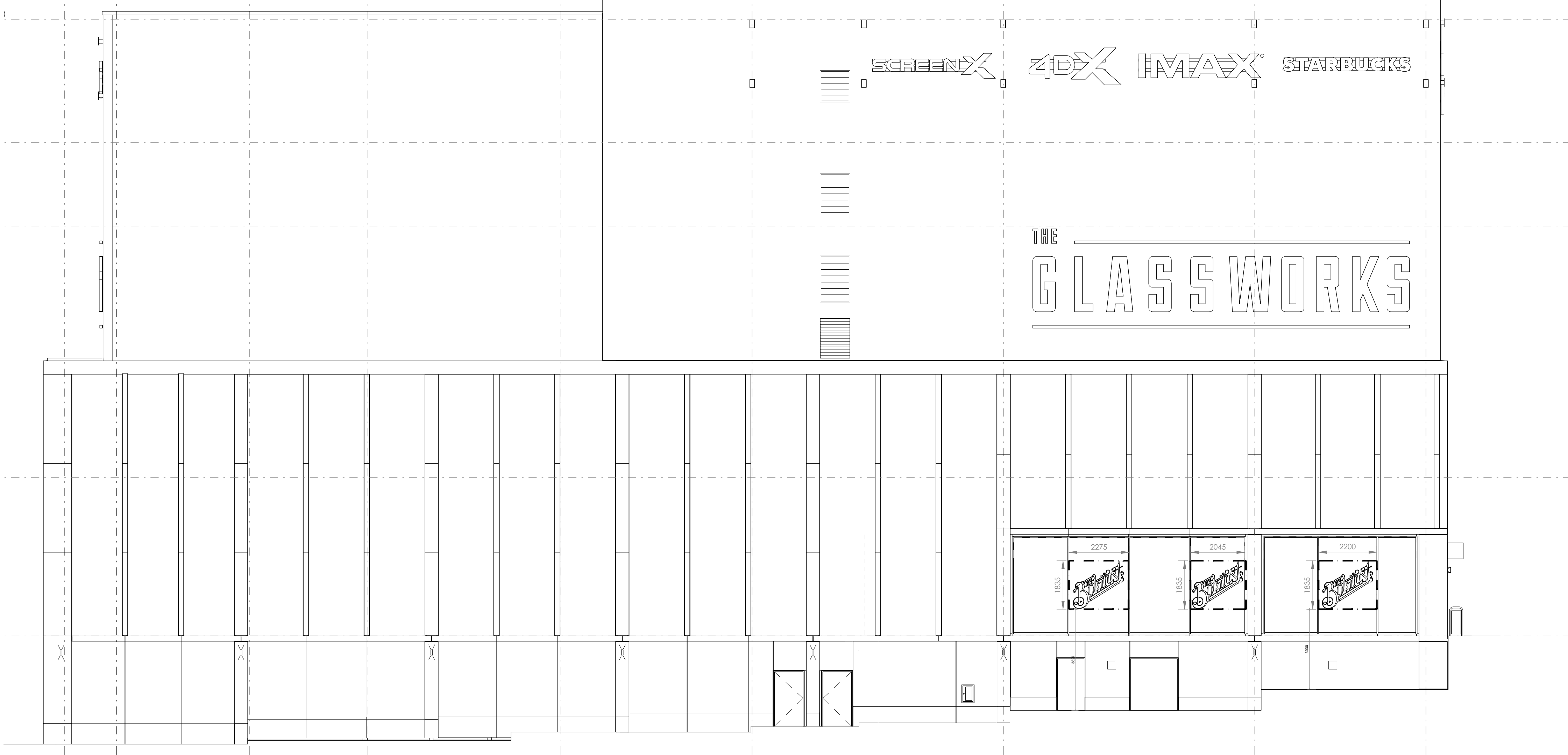
Proposed North Side Elevation, 1:100
