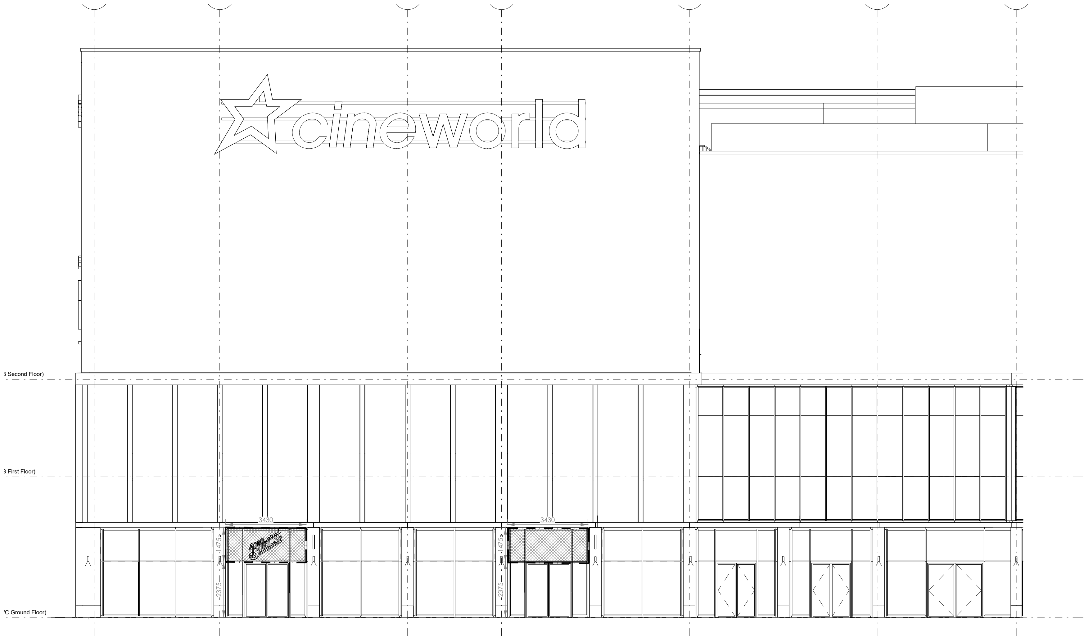
Proposed West Side Elevation, 1:100
