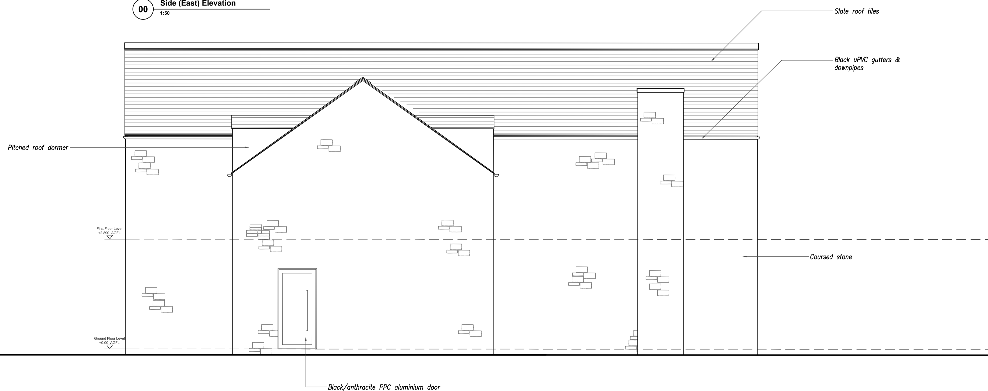
00 Side (West) Elevation 1:50
