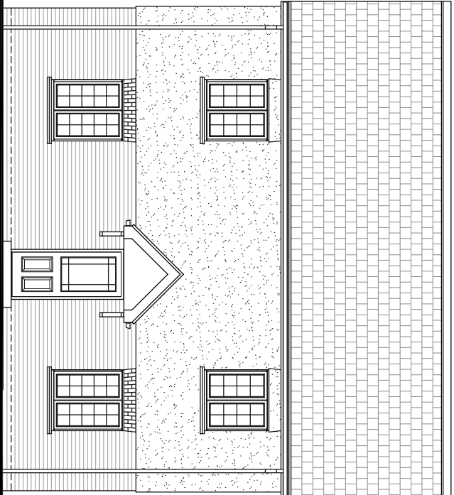
FRONT /SIDE ELEVATION
