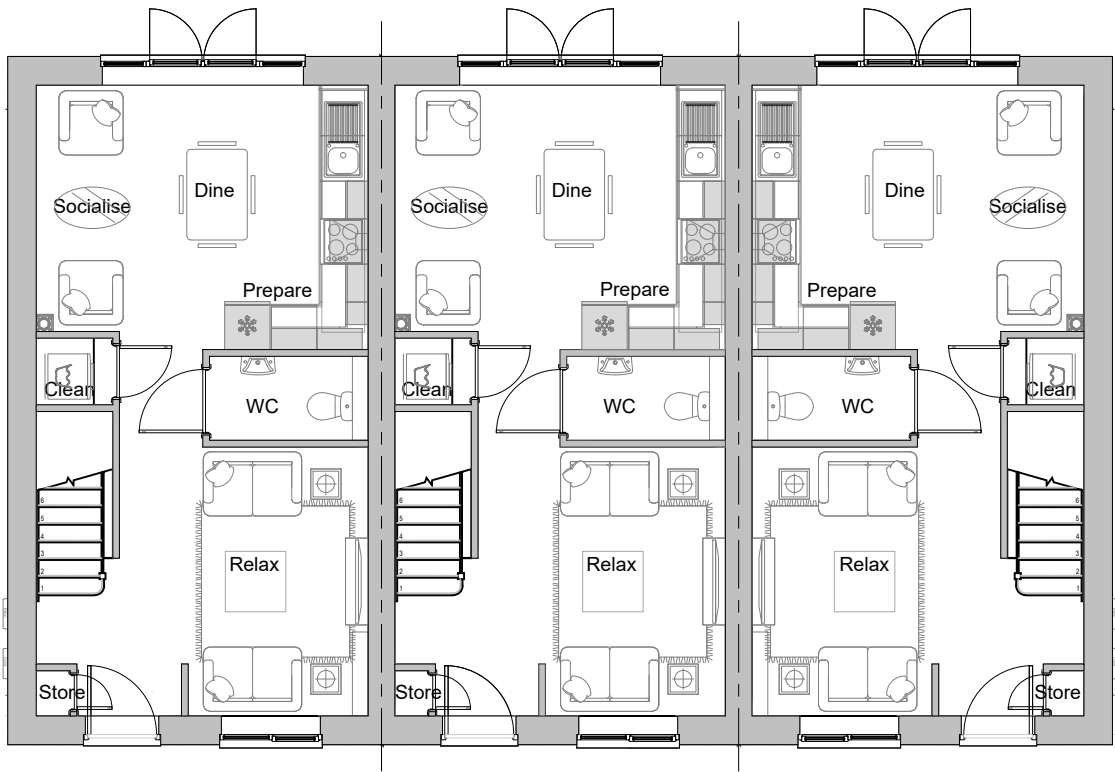
GROUND FLOOR
