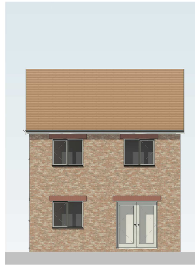
4 | HTE REAR_Elevation 1 : 100
