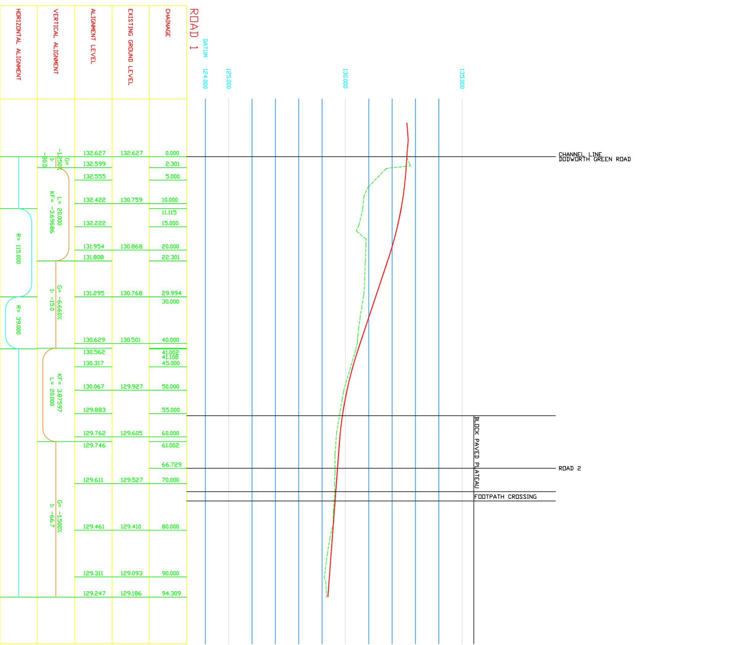
Road Longsection Scale 1:500 Hor 1:100 Ver
