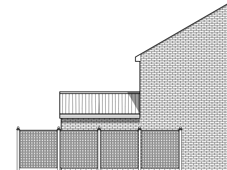
Part Side Elevation facing adjacent Property as Proposed
