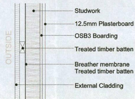
WALL CONSTRUCTION Scale 1:10
