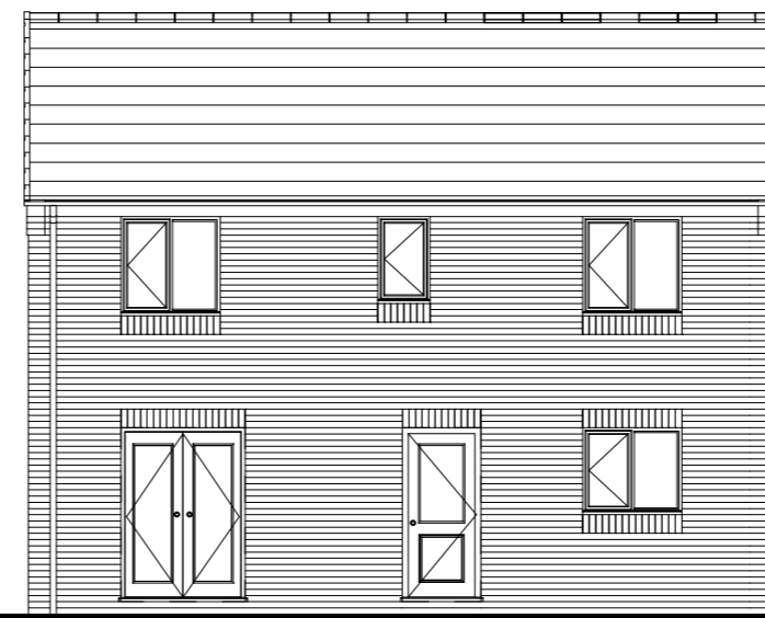
REAR ELEVATION
