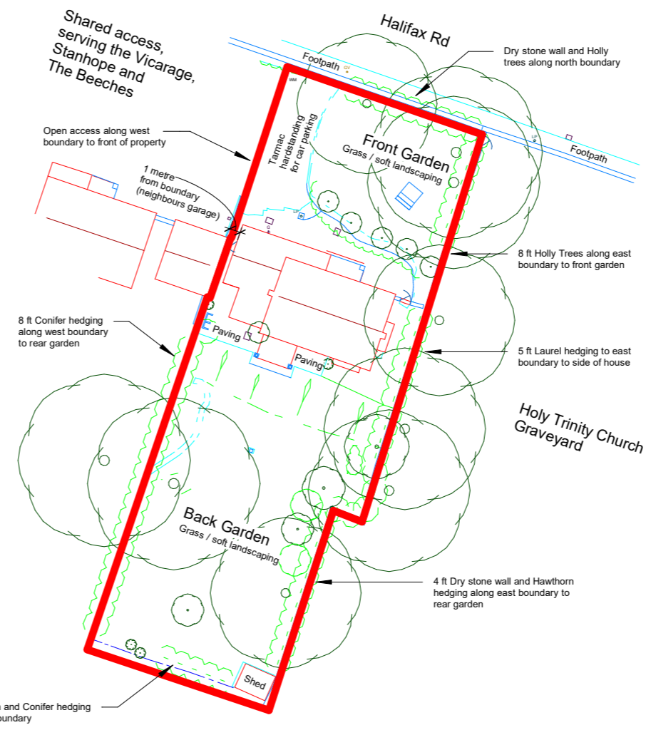
1 Block Plan (with boundaries) 1 : 500
