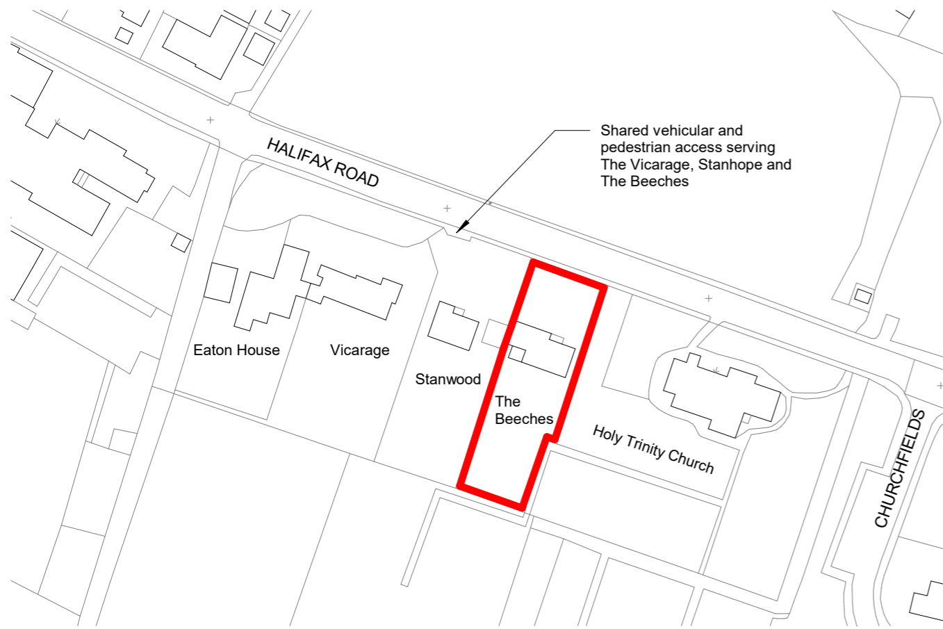
2 Location Plan 1 : 1250
