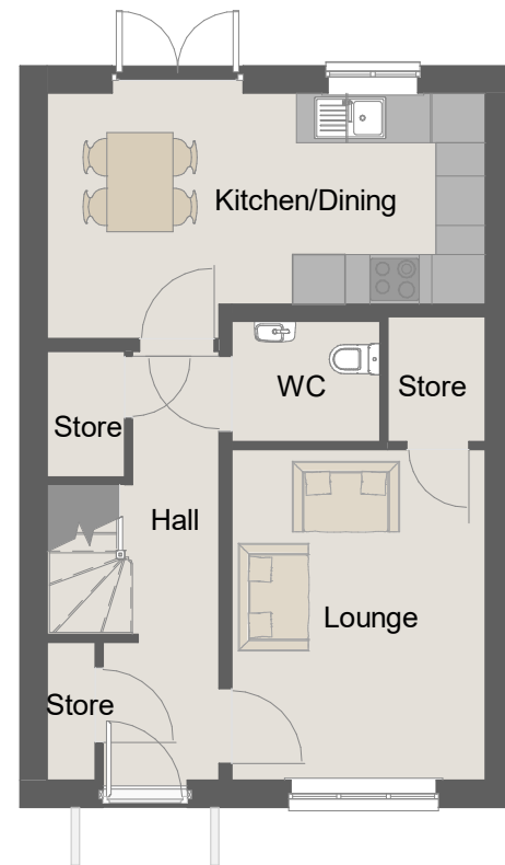
Ground Floor. 1 : 100
