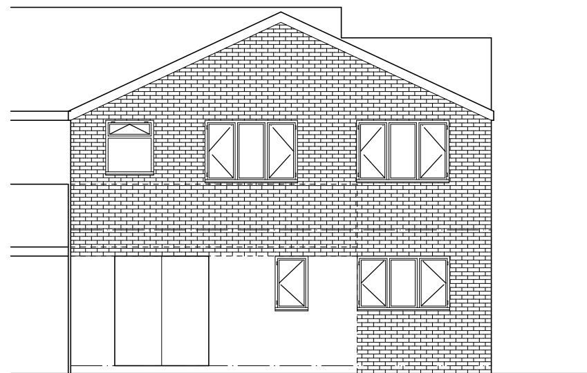
REAR ELEVATION
