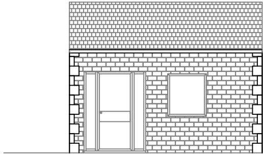
FRONT ELEVATION VIEW ON 'D'
