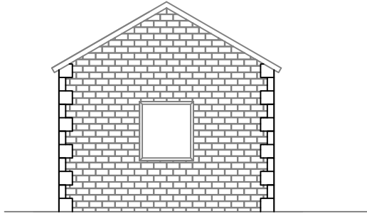
END ELEVATION VIEW ON 'A'
