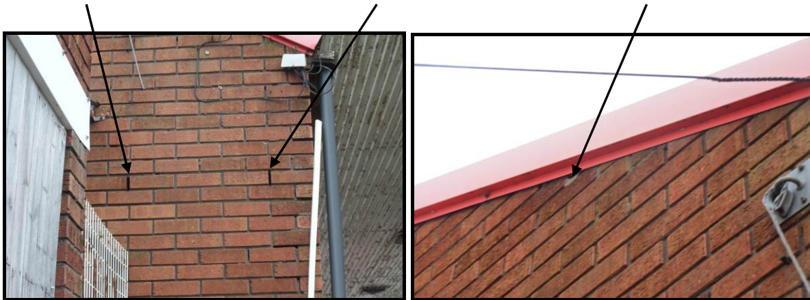
Figure 15. Building B has holes in wall leading to cavity.
