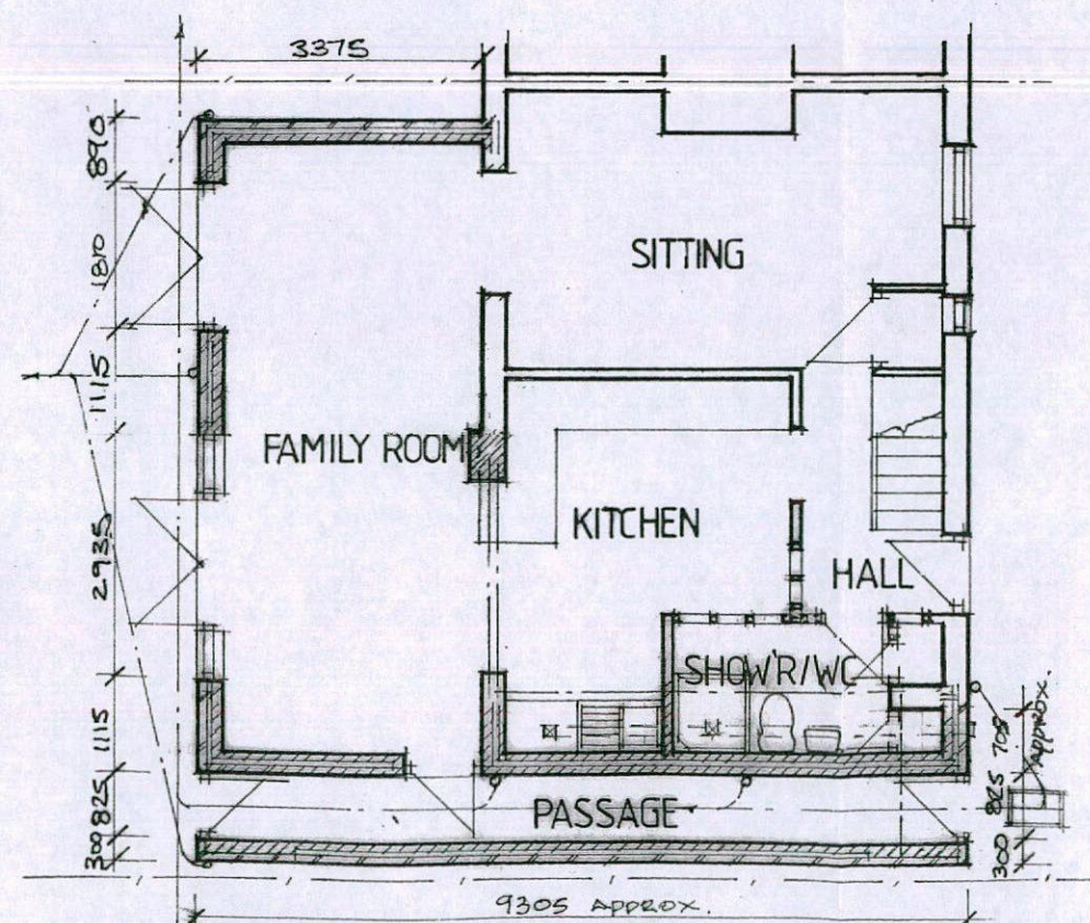
PROP. G.F. PLAN (1:100)
