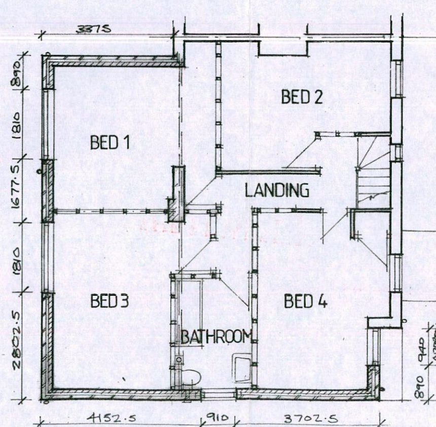
PROP. F.F. PLAN (1:100)
