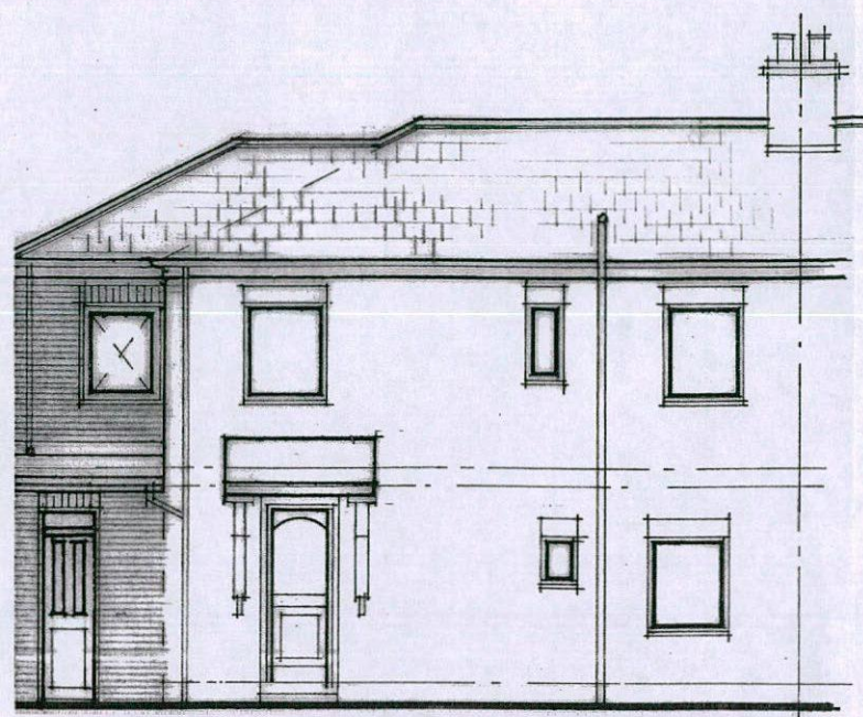
PROP. FRONT ELEVATION (1:100)
