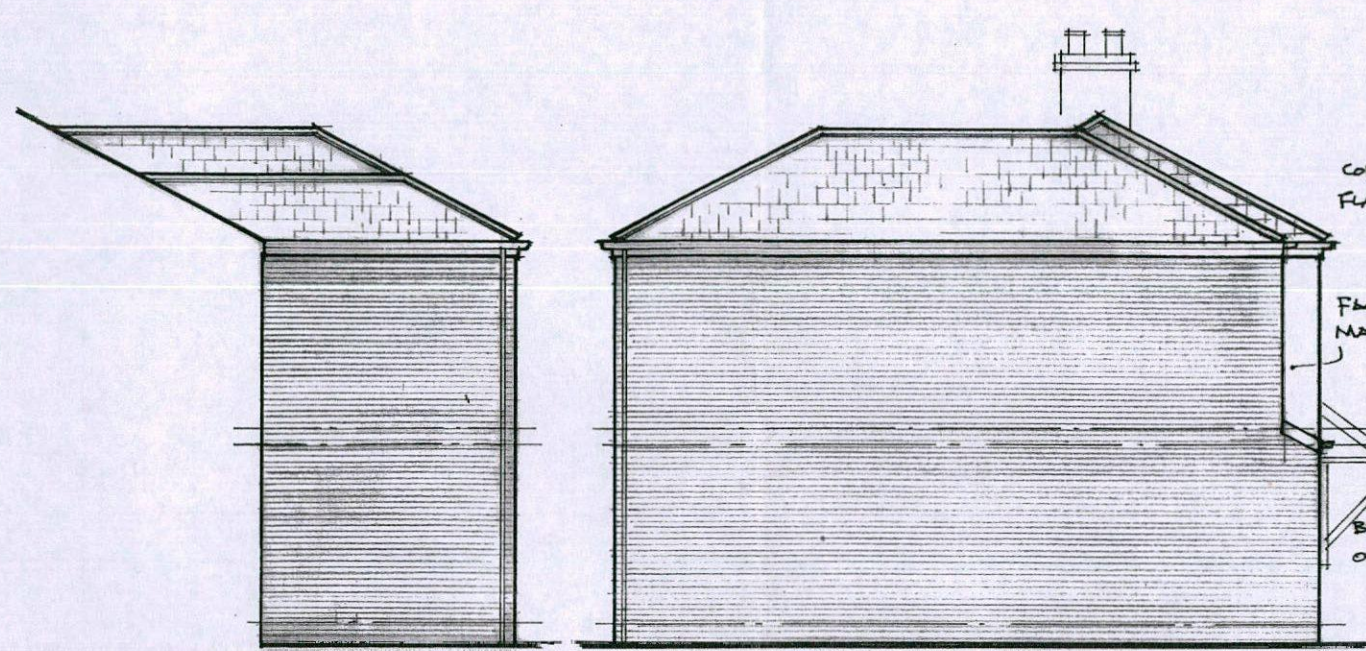
PROP. SIDE ELEVATIONS (1:100)
