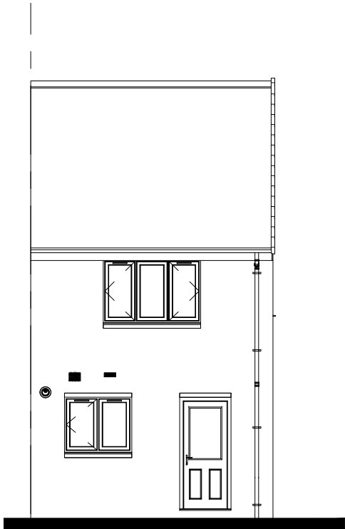
Rear Elevation.
