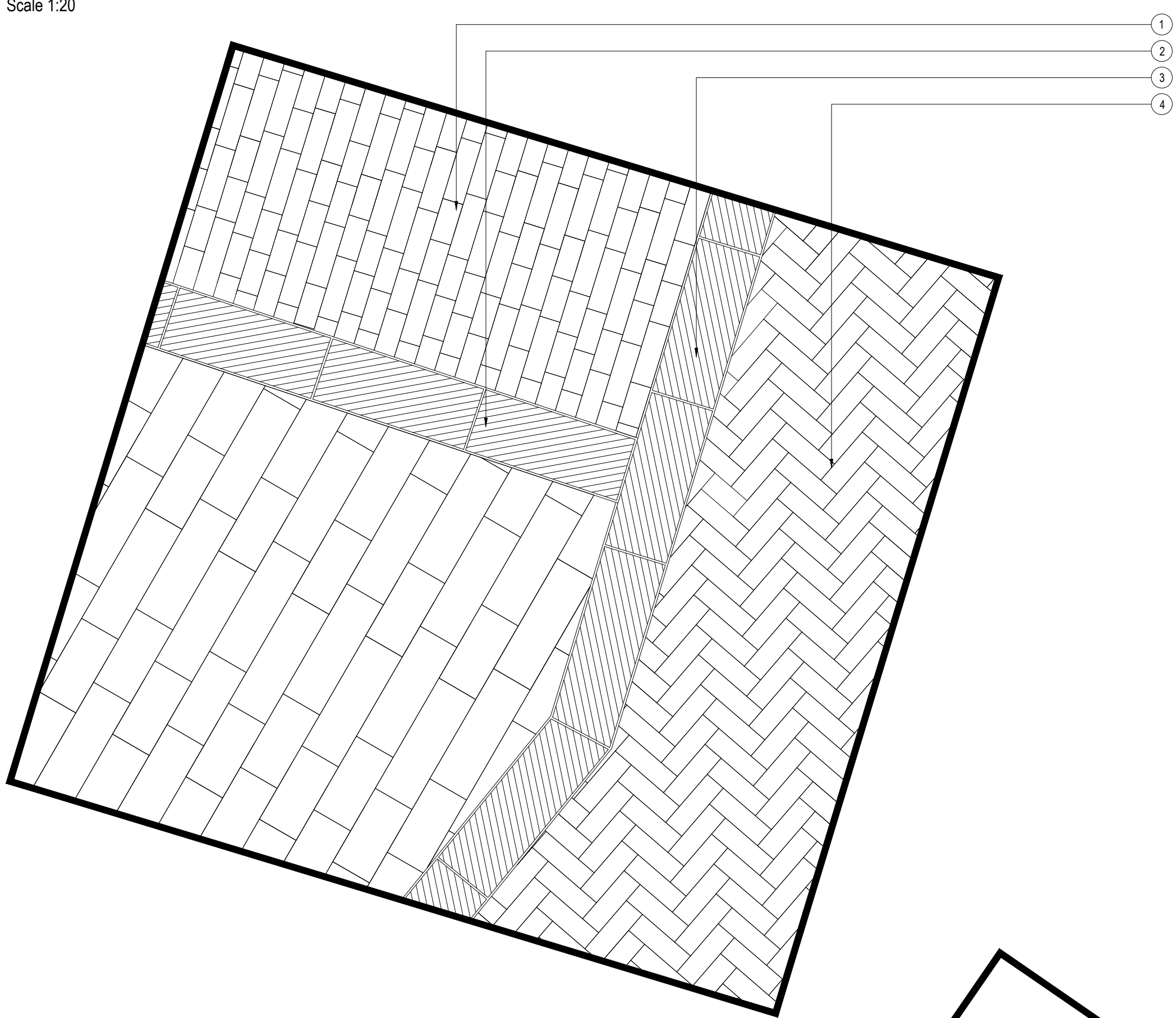
Paving Pattern Ref 2.7 - P3, K1, P4 & P12 Scale 1:20
