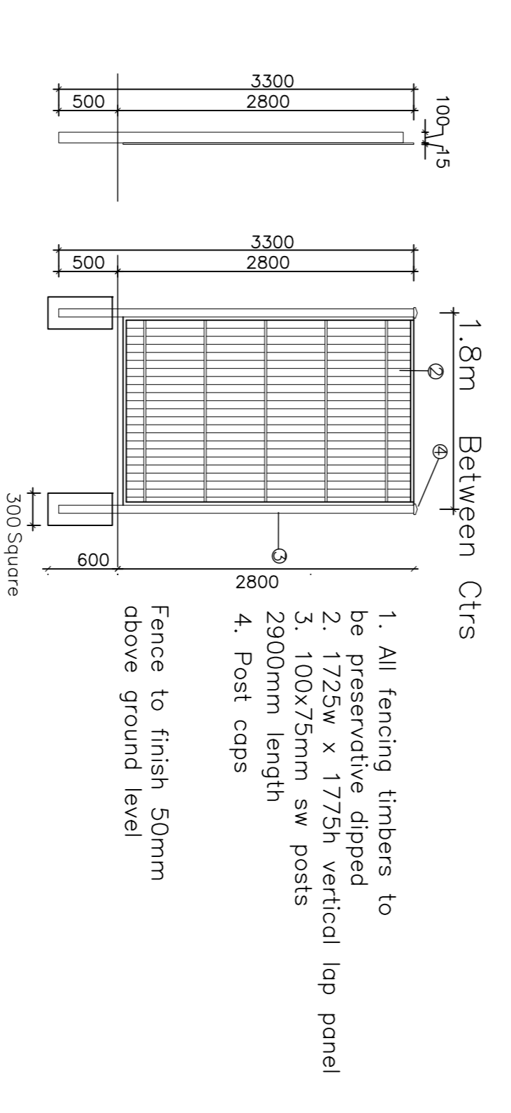
DETAIL 1:50
