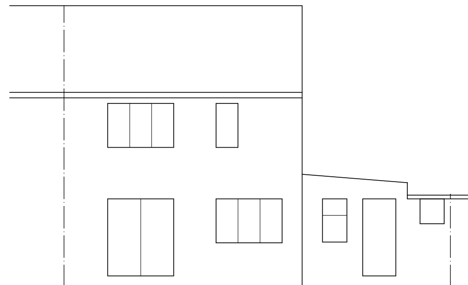
REAR ELEVATION
