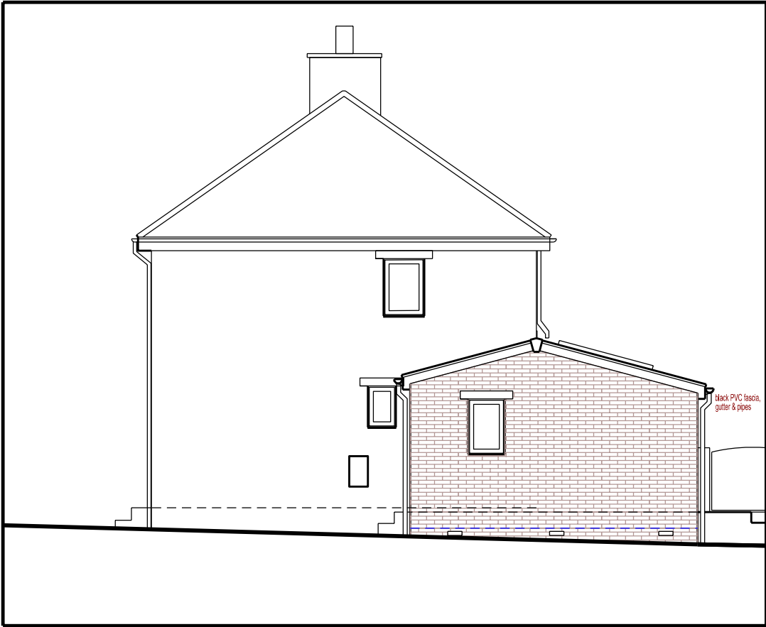
East Elevation - Proposed
