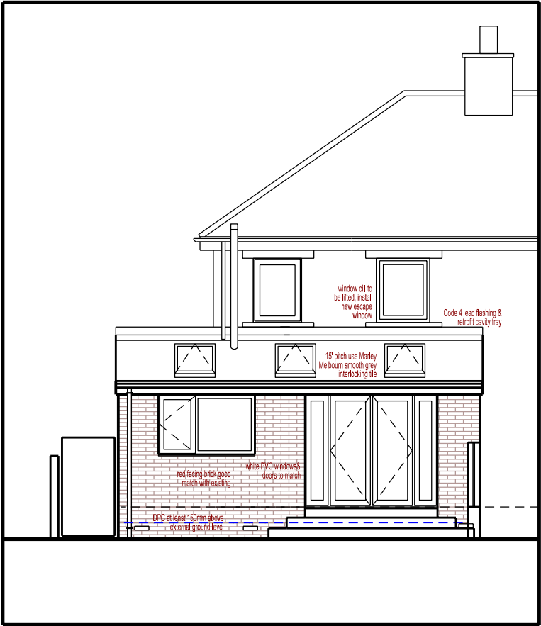
North Elevation - Proposed
