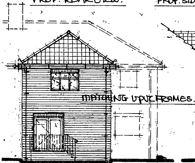
PROP. REAR VIEW.
