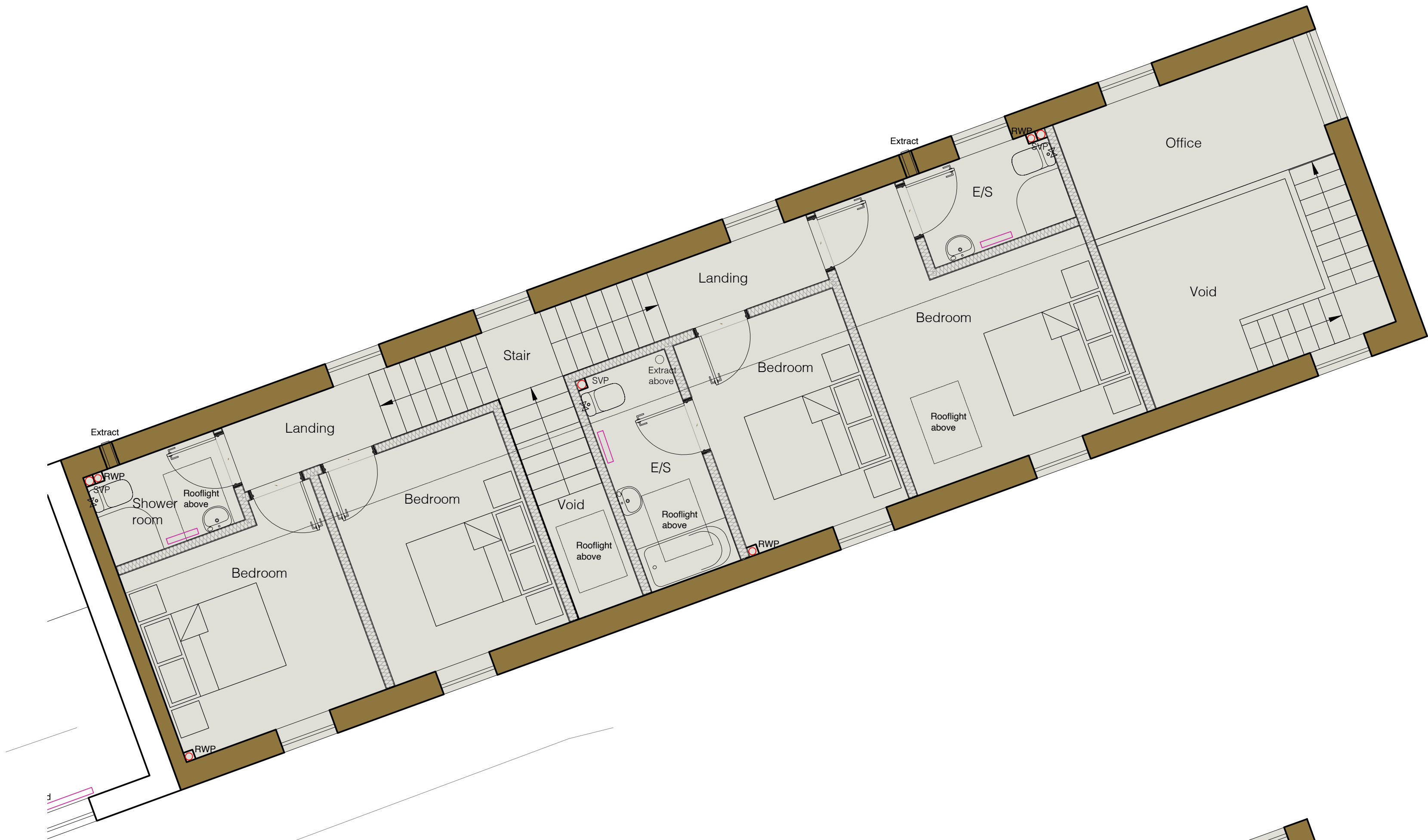
1st Floor
