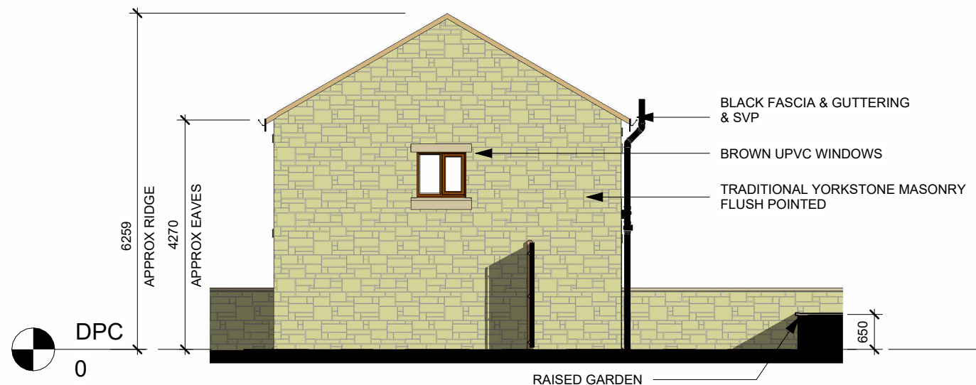
Right Side Elevation 1 : 100
