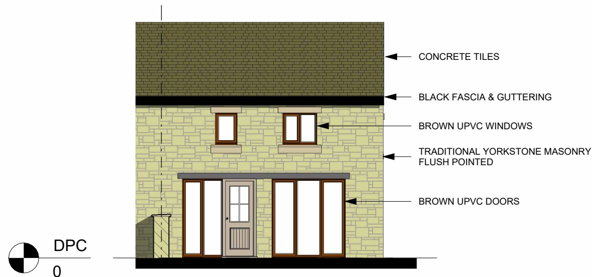
Front Elevation 1 : 100
