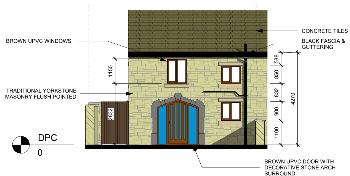
Rear Elevation 1 : 100
