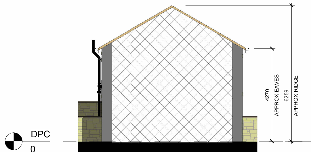
Left Side Elevation 1 : 100
