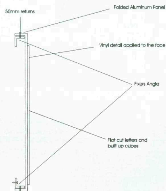
Cross Section for the Flat Di bond panel Panels post sign
