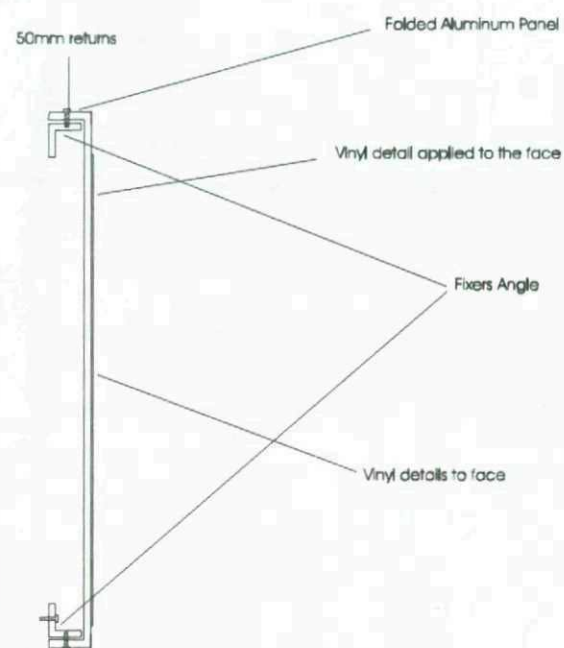
Cross Section for the Folded Aluminum Panels
