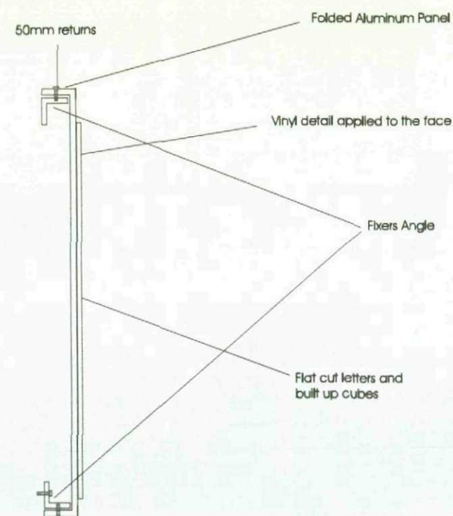
Cross Section for the Folded Aluminum Panels
