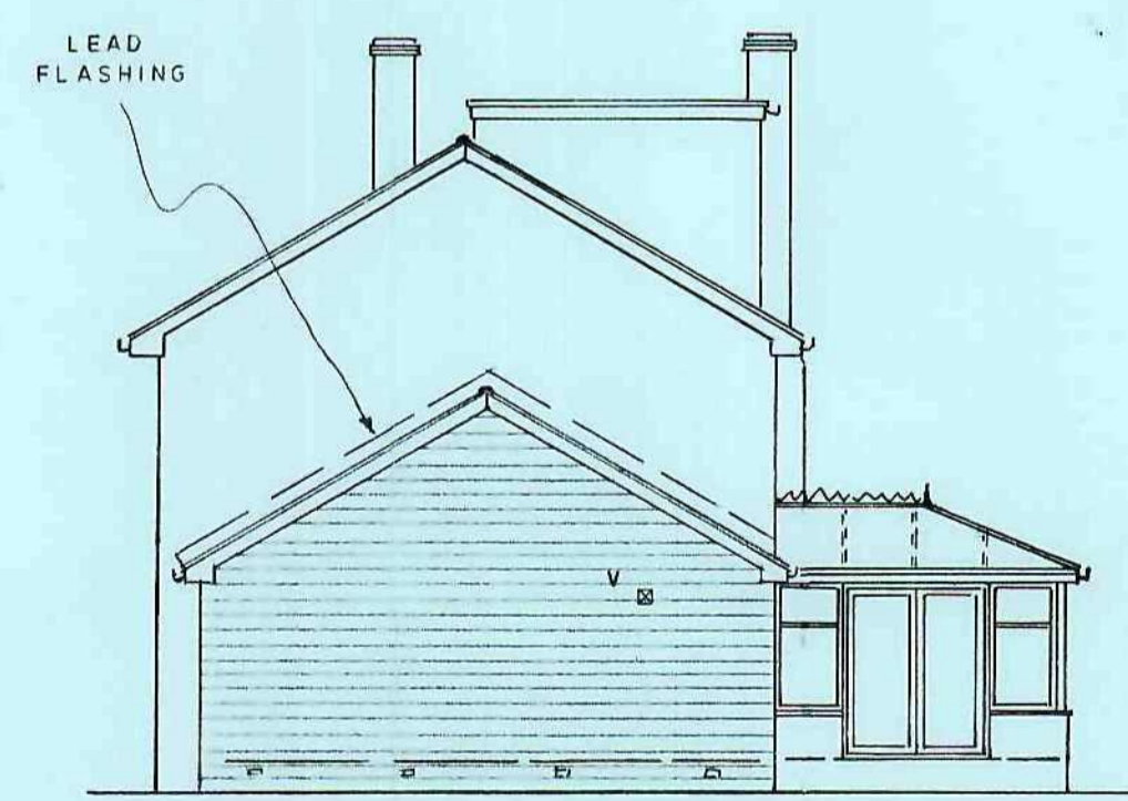
PROPOSED SIDE
