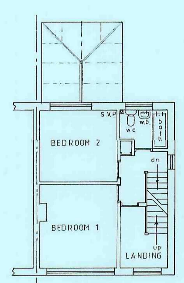
EXISTING F.F. PLAN
