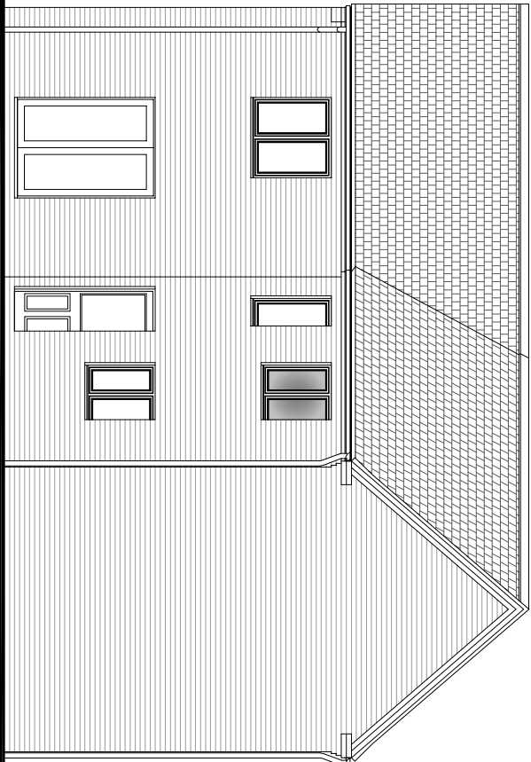
Rear/Side Elevation
