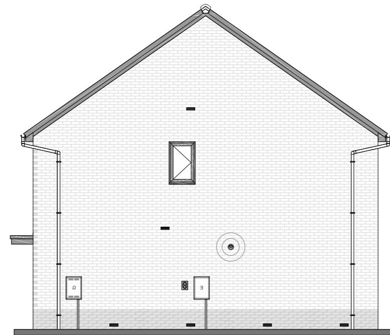
LEFT ELEVATION
