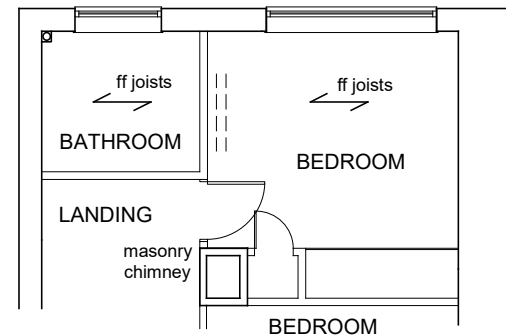
EXISTING PART FIRST FLOOR PLAN
