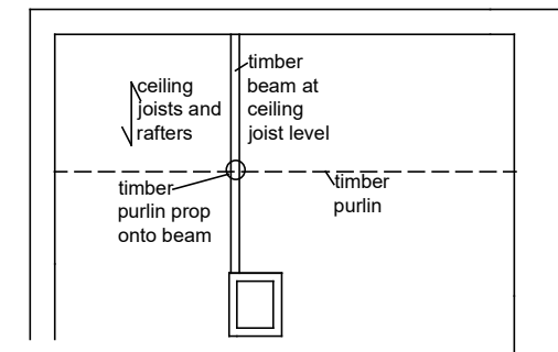
EXISTING PART ROOF PLAN
