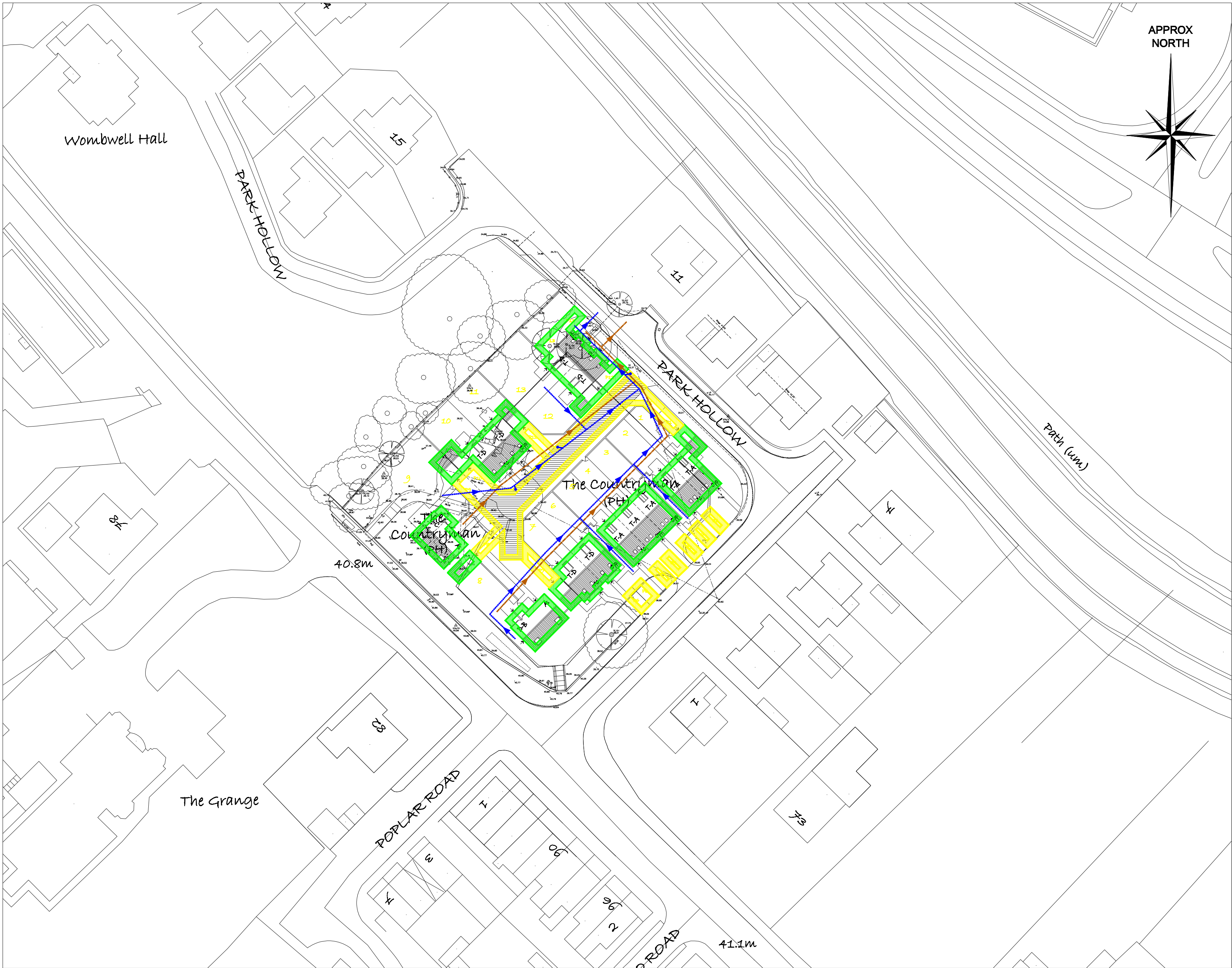
PROPOSED DRAINAGE Scale 1:500
