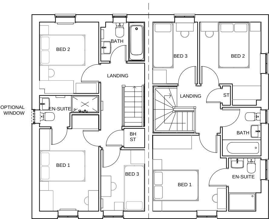
FIRST FLOOR PLAN MAIDSTONE MORESBY
