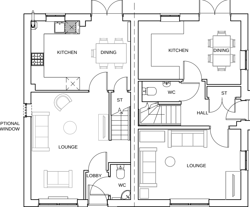
GROUND FLOOR PLAN MAIDSTONE MORESBY
