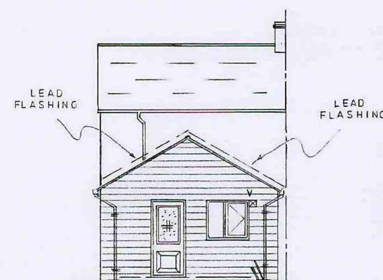
PROPOSED REAR
