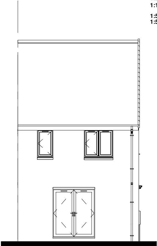
Rear Elevation. 1 : 100
