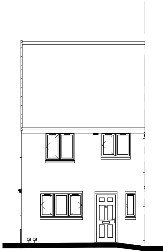
Front Elevation. 1 : 100
