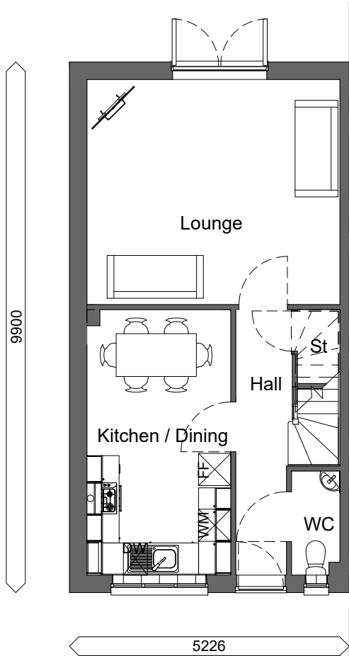
Ground Floor. 1 : 100
