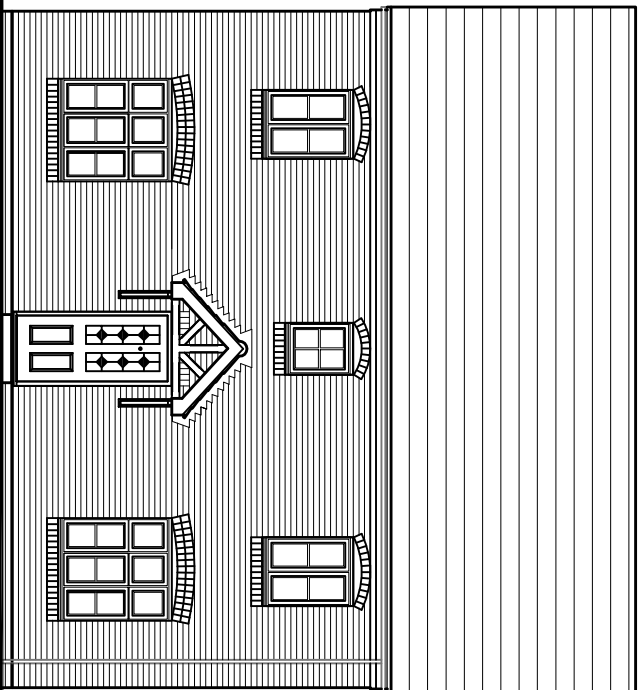
FRONT ELEVATION
