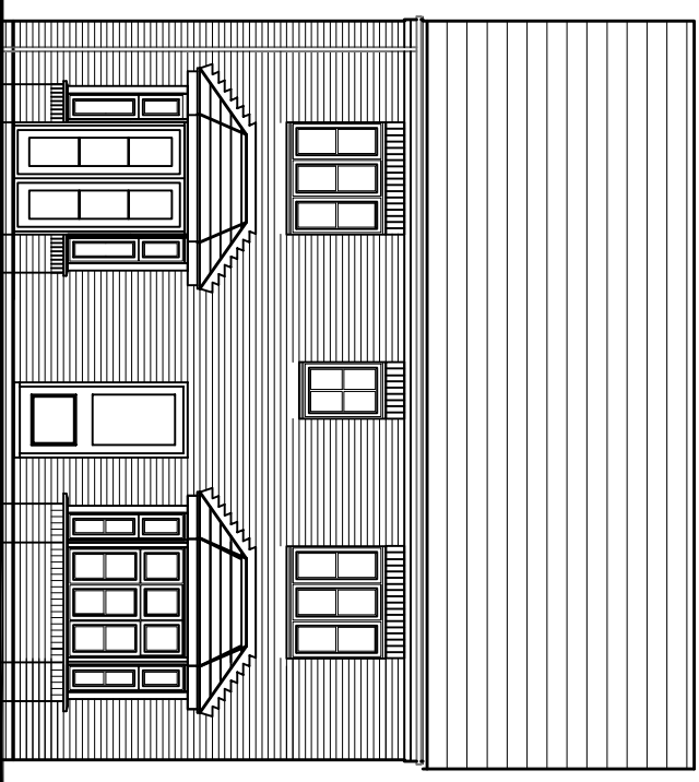
REAR ELEVATION
