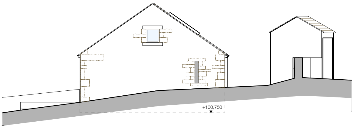
South Elevation 1:100
