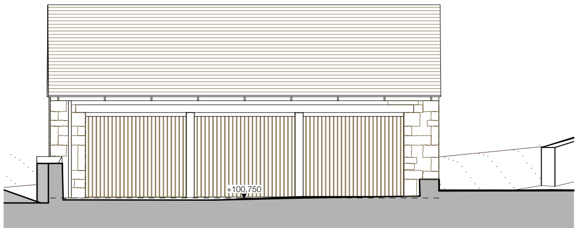
West Elevation 1:100
