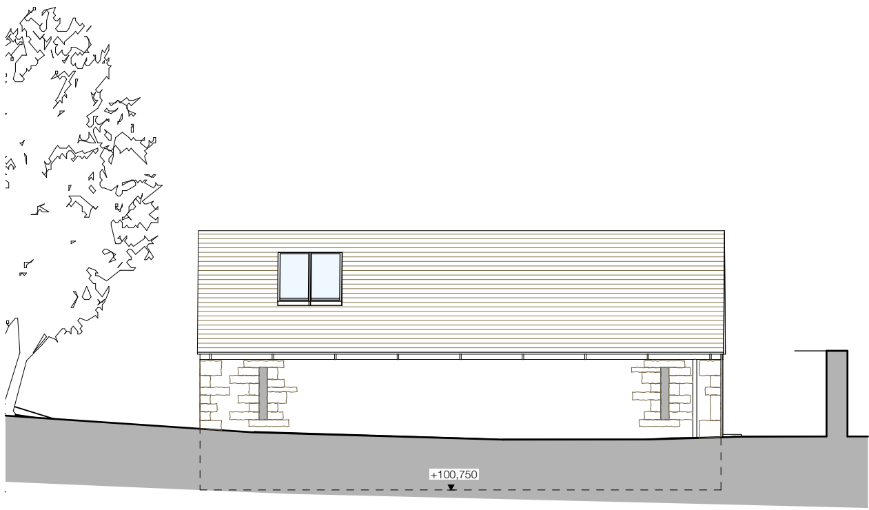
East Elevation 1:100
