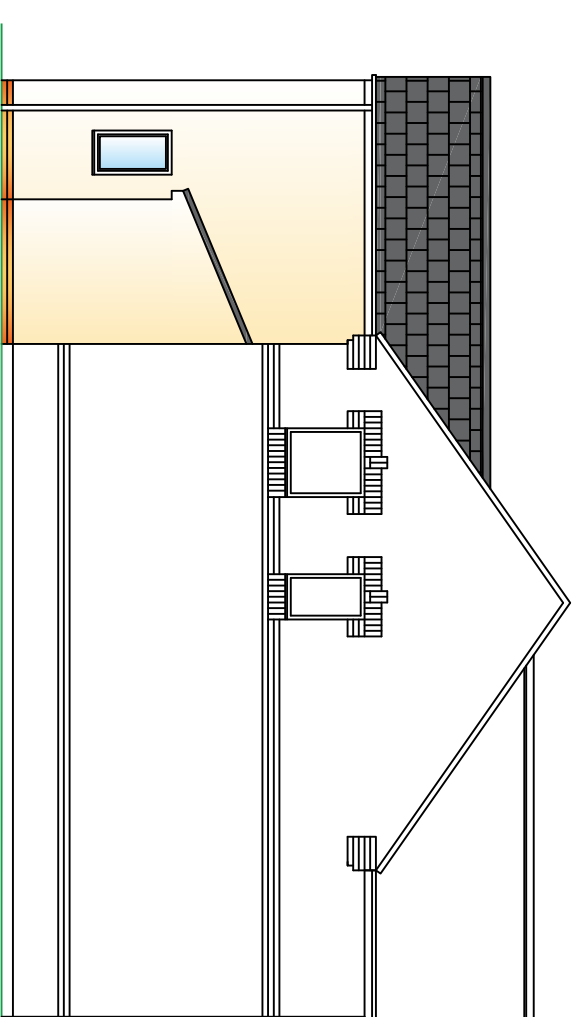
Side Elevation
