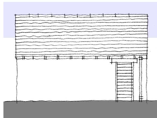
UNIT 1 GARAGE - WEST ELEVATION UNIT 2 GARAGE - SOUTH ELEVATION
