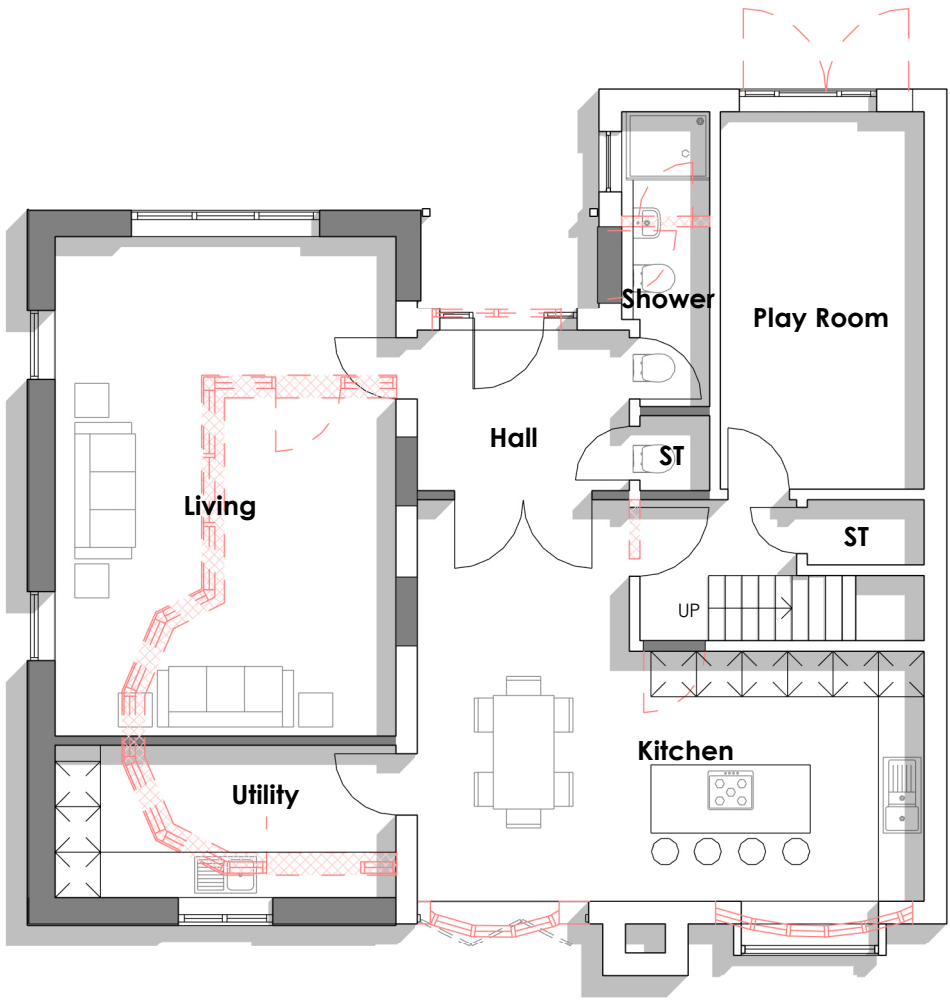
Proposed Ground Floor 1 : 100
