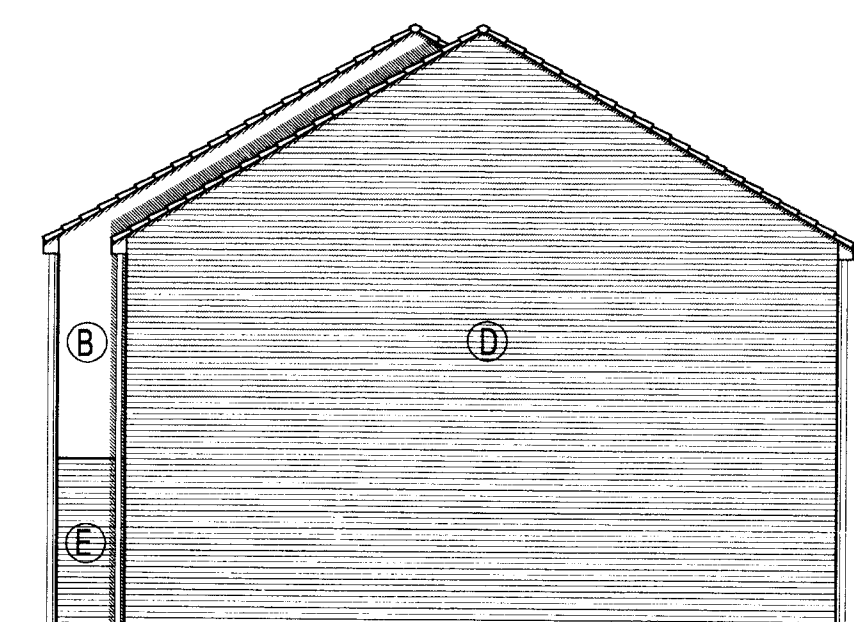
Plot 4 - Gable
