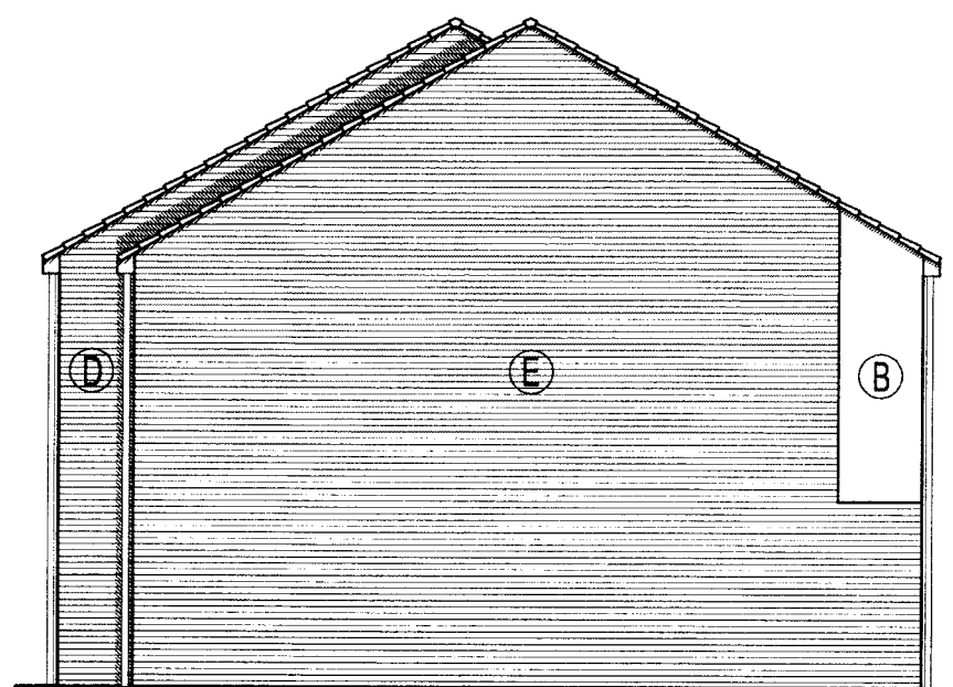
Plot 3 - Gable
