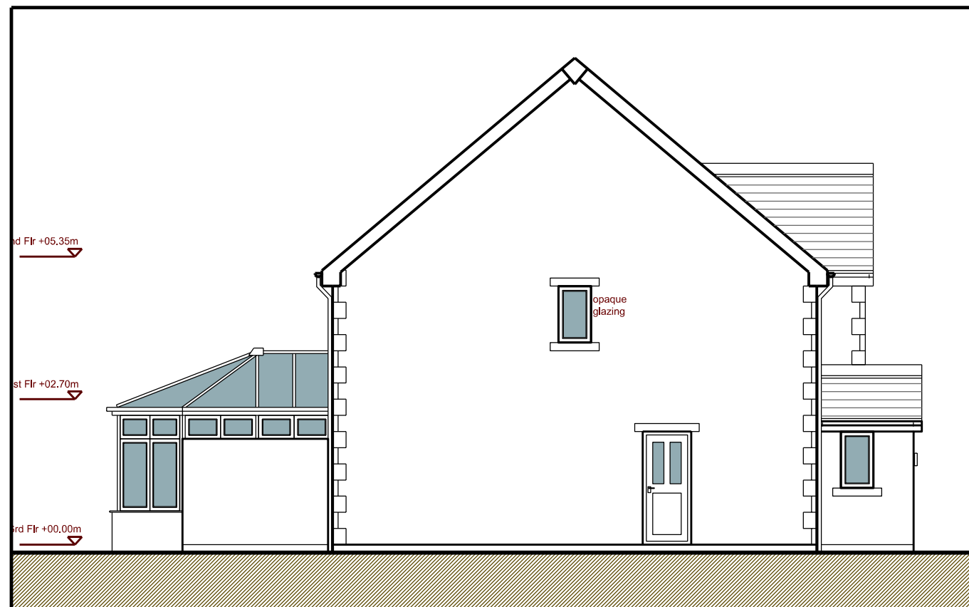
South Elevation
